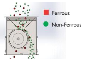
Drum magnet
