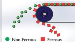
Pulley magnet
